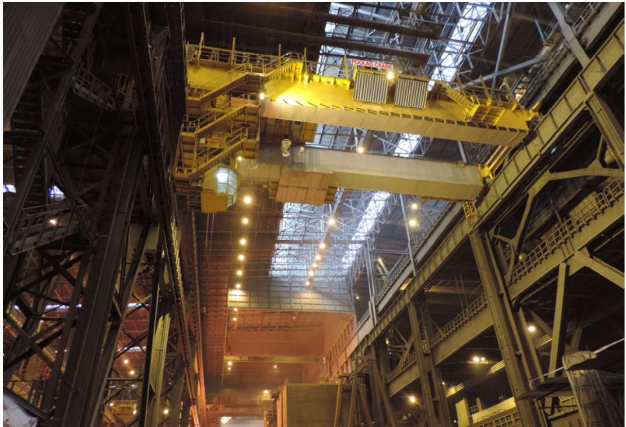
Installation and delivery of crane at site without shutting down the site with highest safety possible
